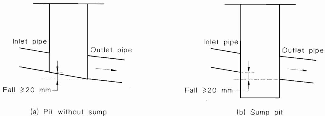
FIGURE 8.4 PIT ARRANGEMENTS
