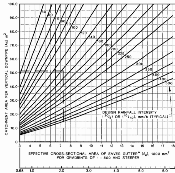
TOTAL FLOW IN EAVES GUTTER (L/s)
