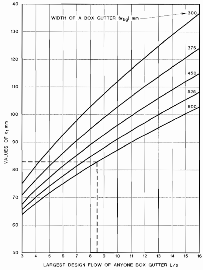
FIGURE I8 REQUIRED SIZE OF SUMP/HIGH-CAPACITY OVERFLOW DEVICE
